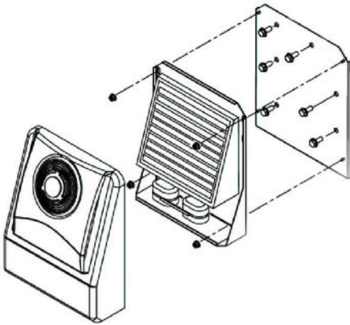
Condenser with cover mounted on backwall of the truck
