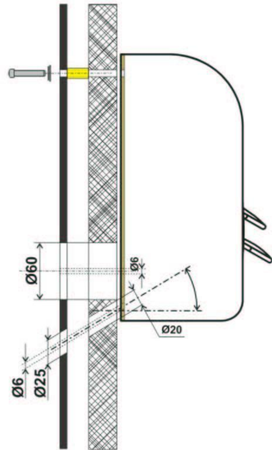
Evaporator mounting criteria
